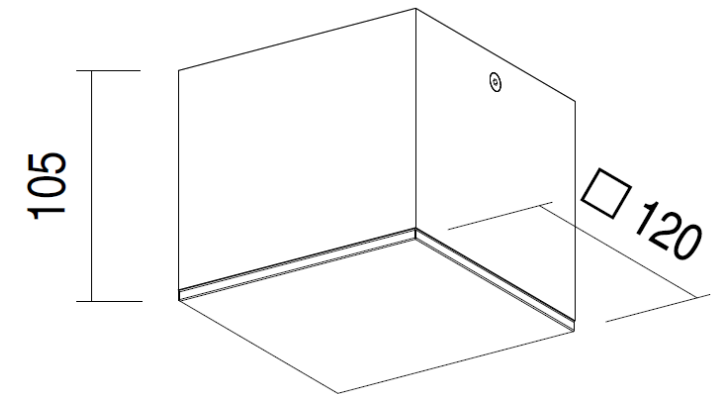
TUBE OUTDOOR 1/2/3
